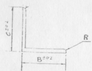
ANGLE MOULDINGS.
