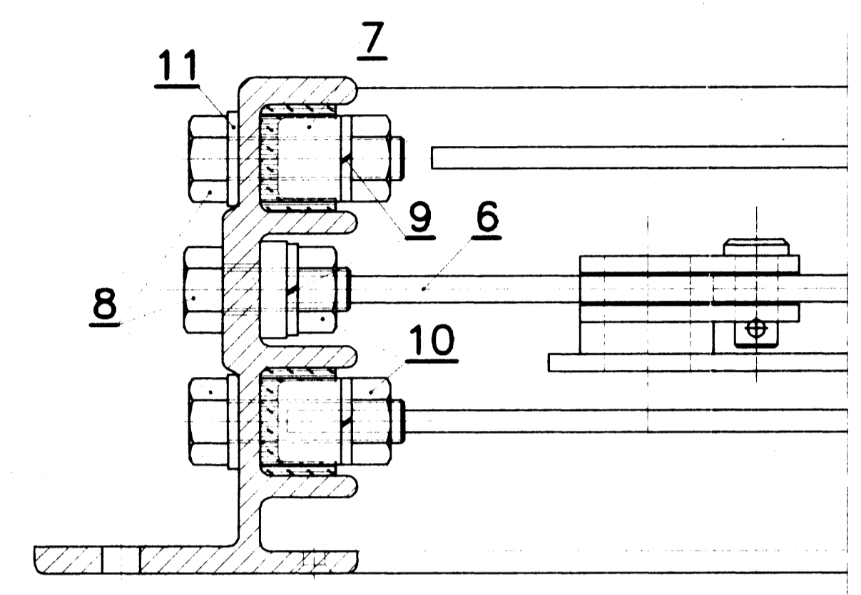
SECTION-CC
