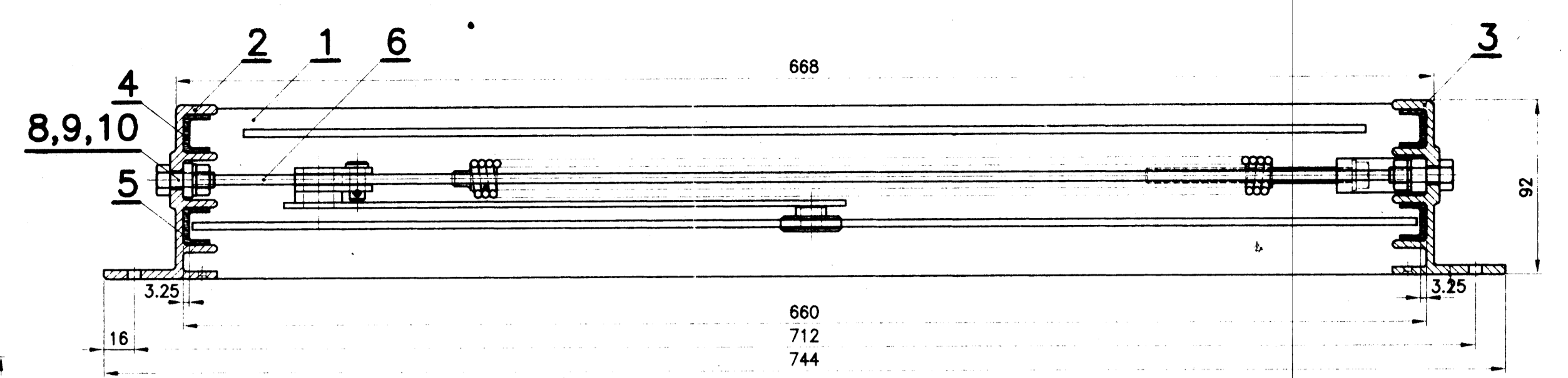
SECTION-BB
