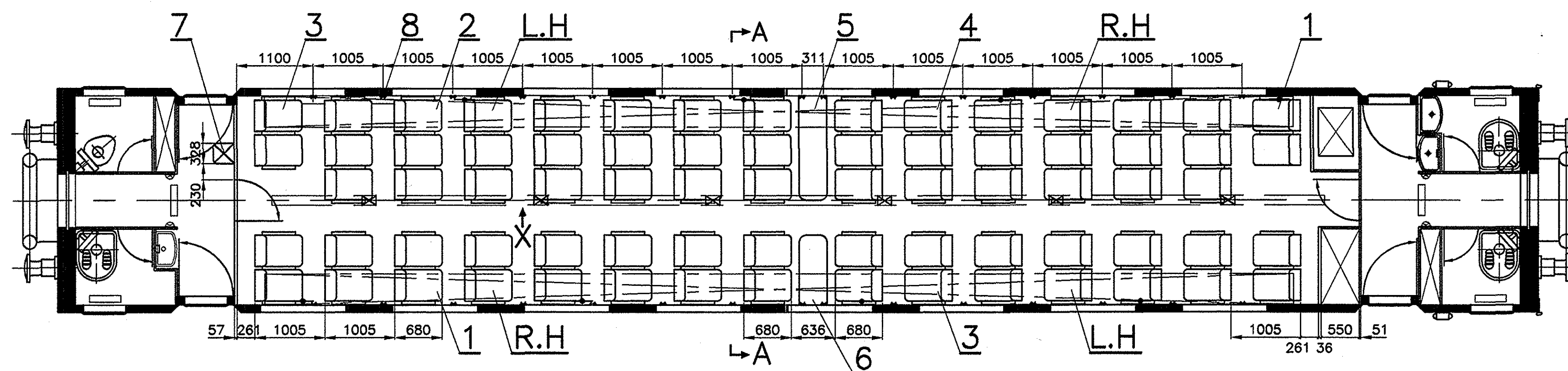
REFERENCE LAYOUT FOR WGSCZAC 8 -9-0-801, WGSCZAC 9 -9-0-901
