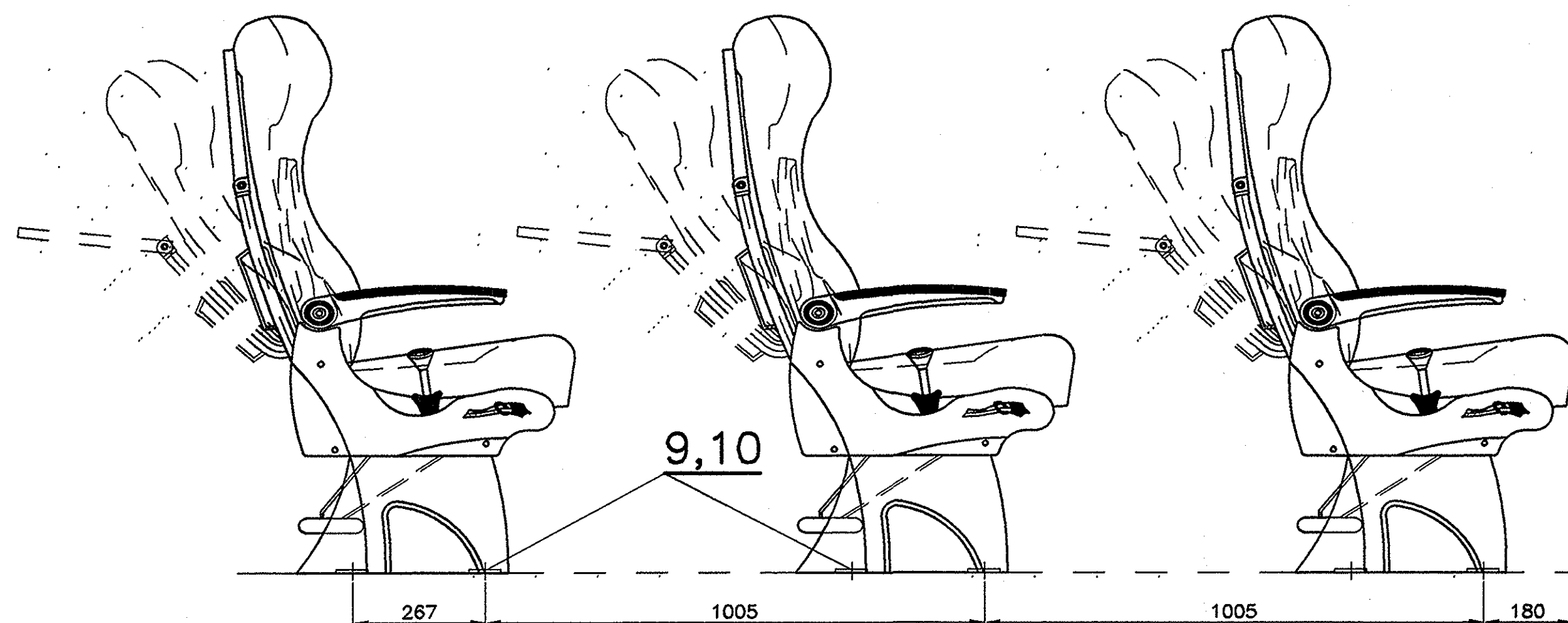
VIEW FROM-X
