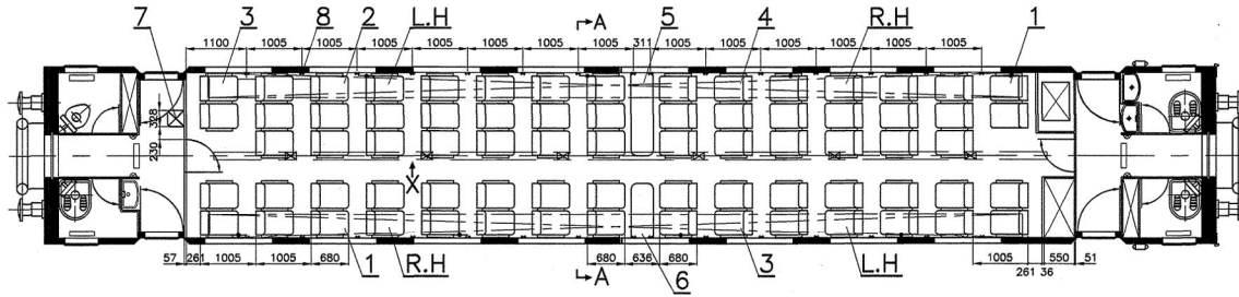
REFERENCE LAYOUT FOR WGSCZAC 8 -9-0-801, WGSCZAC 9 -9-0-901
