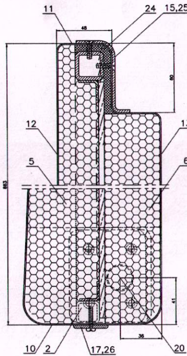
SECTION-CC
