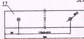
SECTION-EE
