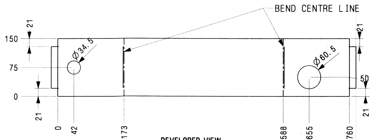
DEVELOPED VIEW (FOR REFERENCE ONLY)
